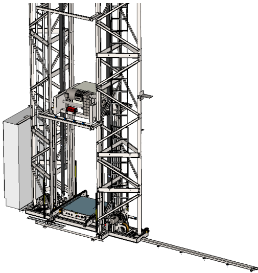
Mimer Crane together with Mimer Satellite
